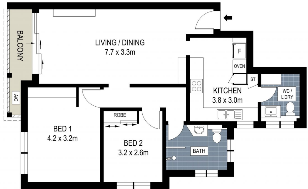
SECOND FLOOR
