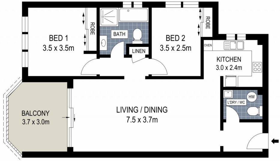
FIRST FLOOR
