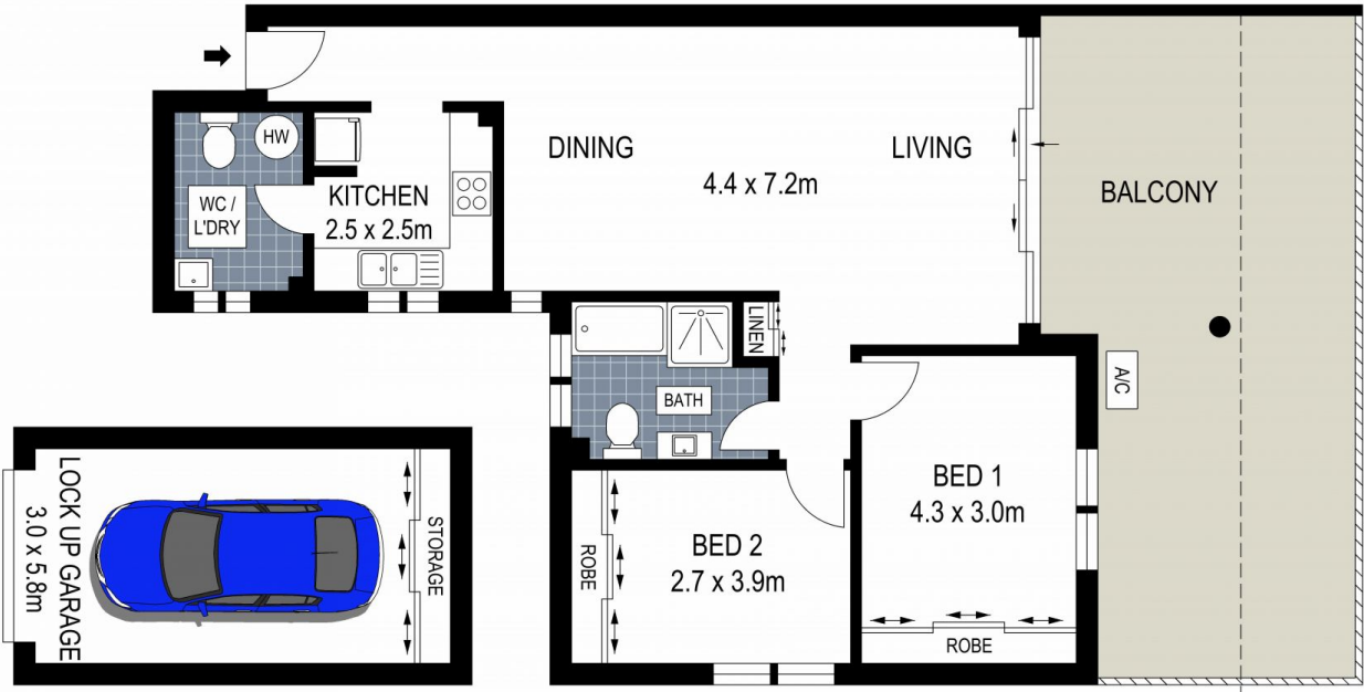
GROUND FLOOR
